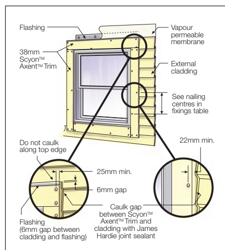
FIGURE 1 19MM AND 38MM SCYON™ AXENT™ TRIM FIXING AROUND WINDOW
